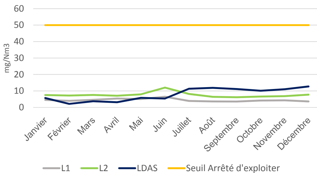
CO 2018
