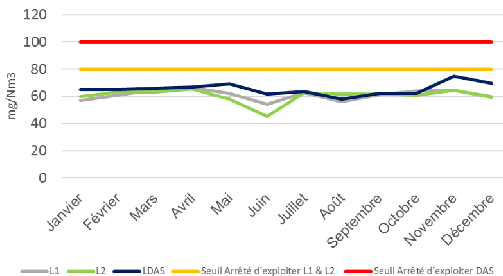
NOx 2018
